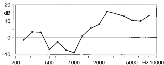
Fig. 8.18 Sound level increase in the direction of sight for the player when raising the bell of the trumpet
