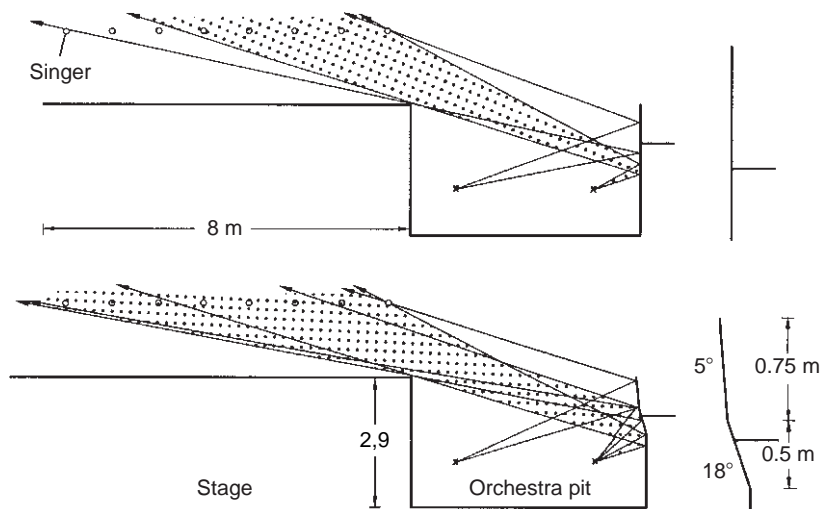
Fig. 6.23 Sound reflections from a deep orchestra pit to the stage, for differently shaped balustrades
